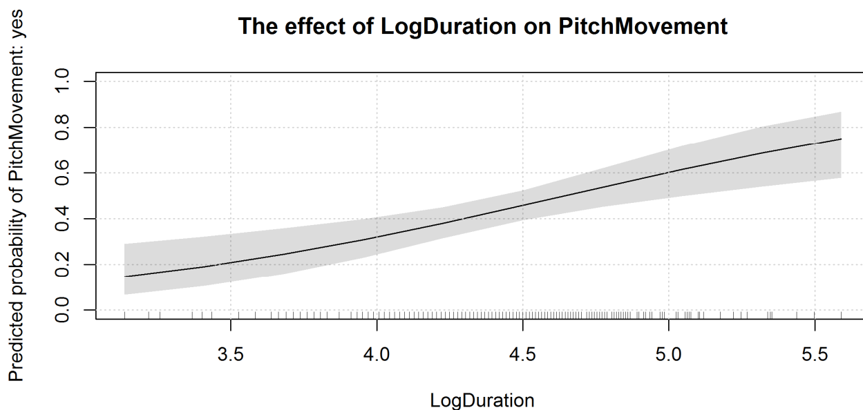
Figure 3. The Log of Vowel Duration’s effect of PitchMovement. Vowel durations are represented on the x-axis, with longer durations to the right and the probability of pitch movement is represented on the y-axis.
