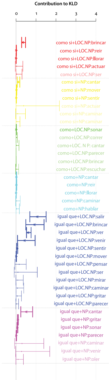
Figure 2. Constructions attracting verb lemmas
